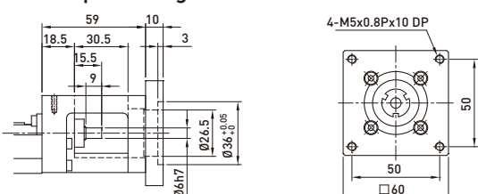
Motor Adaptor Flange F4
