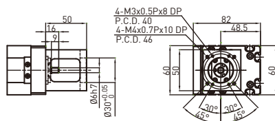
Motor Adaptor Flange F0
