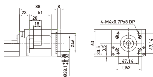
Motor Adaptor Flange F6
