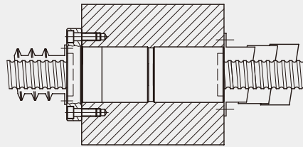
Fig 4.6 Ballscrew protection by telescopic or bellow type covers
