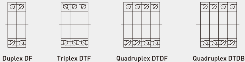
Fig 4.4 Different arrangements of ballscrew support bearings
