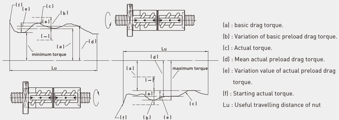
Fig 4.21 Nomenclature of drag torque measurement
