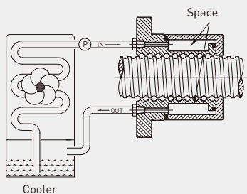
Fig. 8.8 Cool type II with cooler
