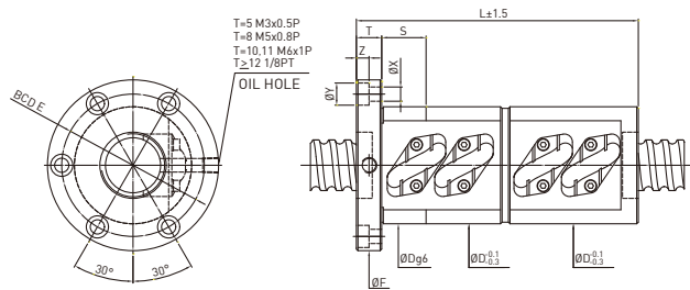
Re-circulation plate below the nut body
