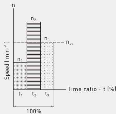
Fig 4.22 Equivalent speed
