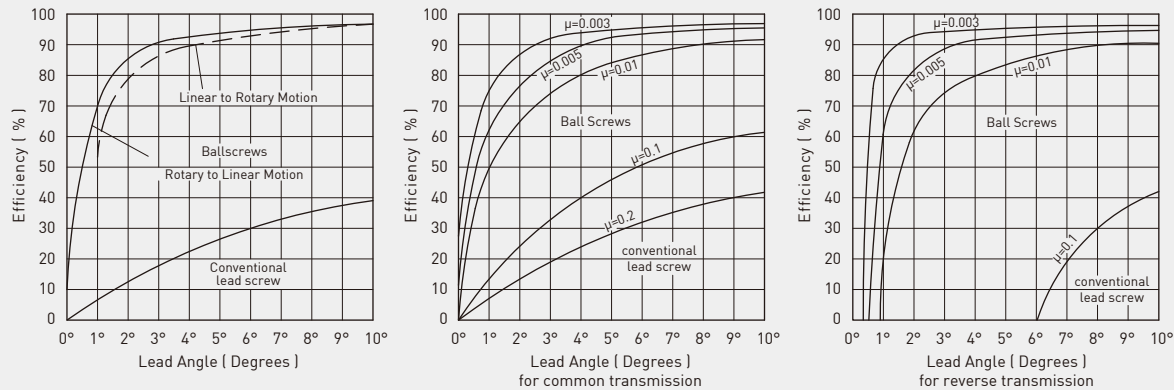
Fig 2.2 Mechanical efficiency of ballscrews
