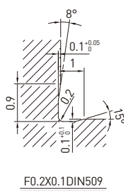
X DETAIL
