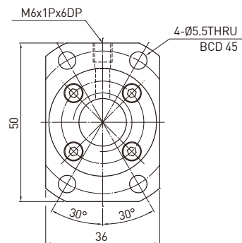
D-D VIEW
