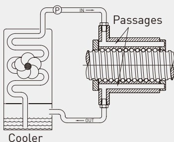
Fig. 8.2 Cool type I with cooler
