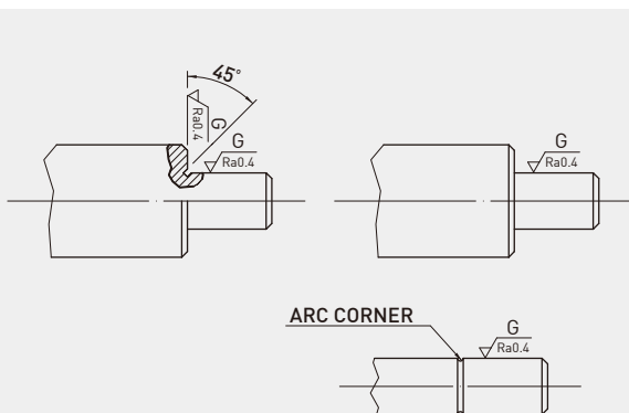
Fig A-2 The design of ballscrew spindle end
