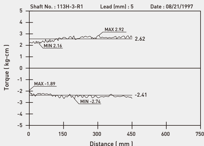
Fig 2.5 HIWIN preload checking diagram
