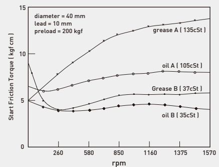
Fig 4.32 The influence of oil viscosity on the friction torque
